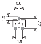
MCP1702T-1502E/CB
