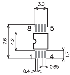
M95M01-DWDW3TP/K
