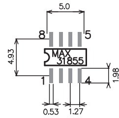
MAX31855KASA+
