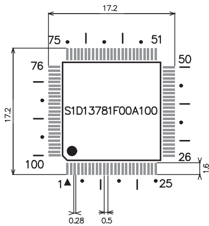
S1D13781F00A100
